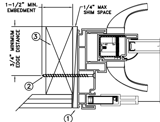
FRAME JAMB SECTION (TYP) HORIZONTAL SECTION
